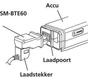
<BT-E6000/BT-E6001>
