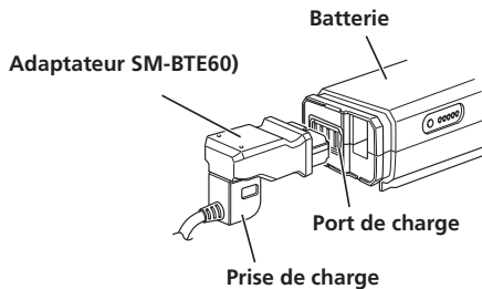
<BT-E6000/BT-E6001>
